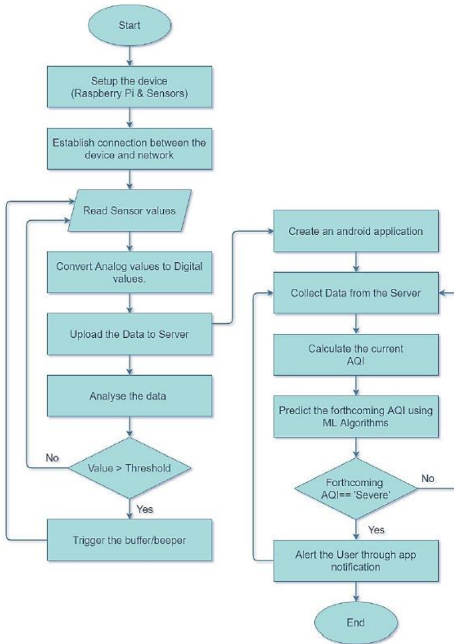
Figure 2: Overall flow of the proposed system.
