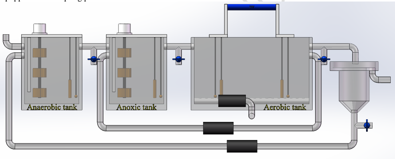
Fig. 1. A 2 O process device.
