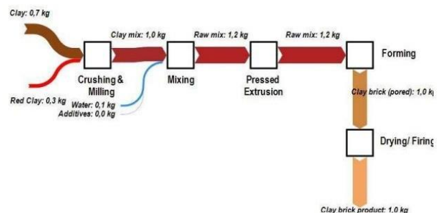
Figure 5. Inventory process flow for brick.
