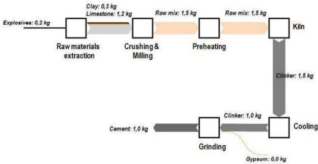
Figure 7. Inventory process flow for cement.
