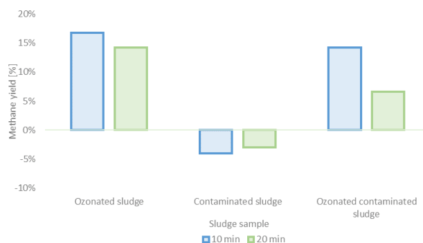
Figure 5. Methane yields of PVC-contaminated (1 g L -1 ) and ozonated sludge at higher ozone dose 3.99 g h -1 (10 and 20 min) in comparison to control sample.
