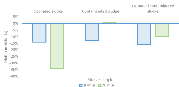
Figure 4. Methane yields of PVC-contaminated (1 g L -1 ) and ozonated sludge at lower ozone dose 3.54 g h -1 (10 and 20 min) in comparison to control sample.
