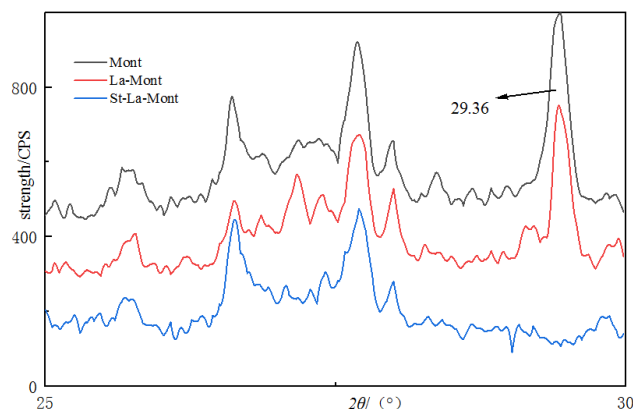
Figure 1. XRD Phenogram.
