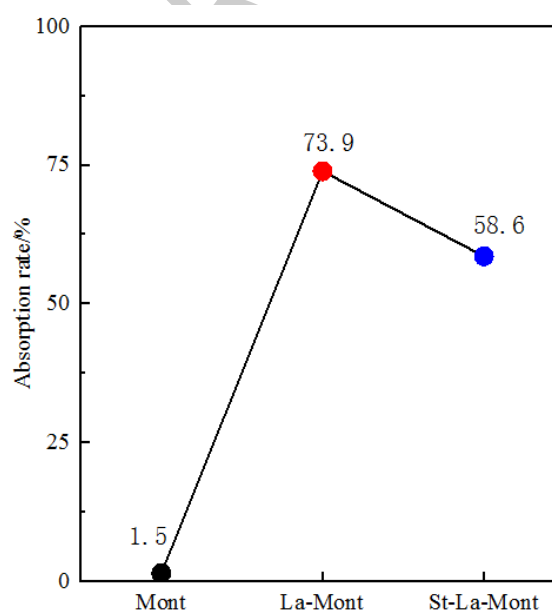
Figure 7. Chromium(VI) adsorption effect of Mont, La-Mont, St-La-Mont.
