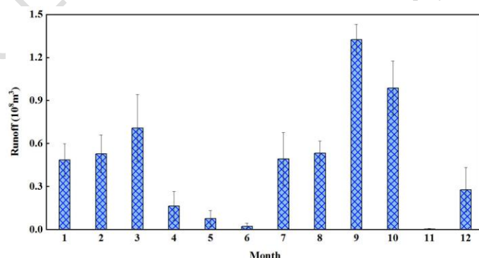
Fig. 3 The monthly variation of runoff after eco-water diversion project in study area
