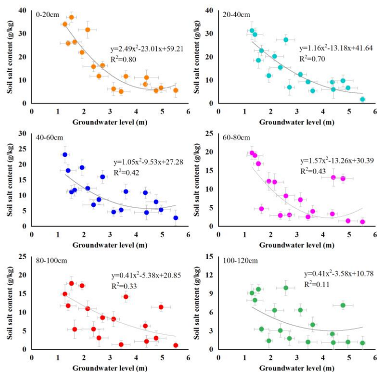
Fig. 8 The relationship between soil salt content and groundwater level
