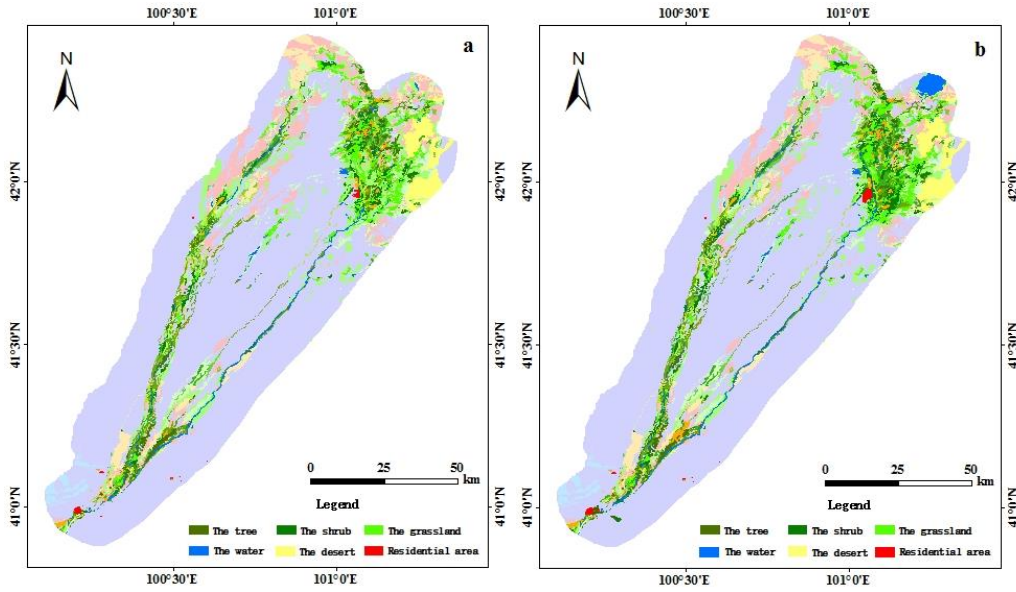
Fig. 9 The spatial change of vegetation in study area(a- before eco-water diversion project; b- after eco-water diversion project)
