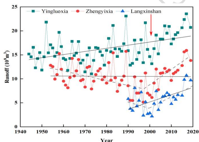
Fig. 2 The annual variation of runoff after eco-water diversion project in study area
