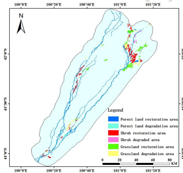
Fig. 10 The degradation area of different vegetations in study area
