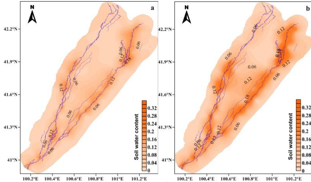
Fig. 4 The spatial change of soil water content in study area (a-before eco-water diversion project; b- after eco-water diversion project)
