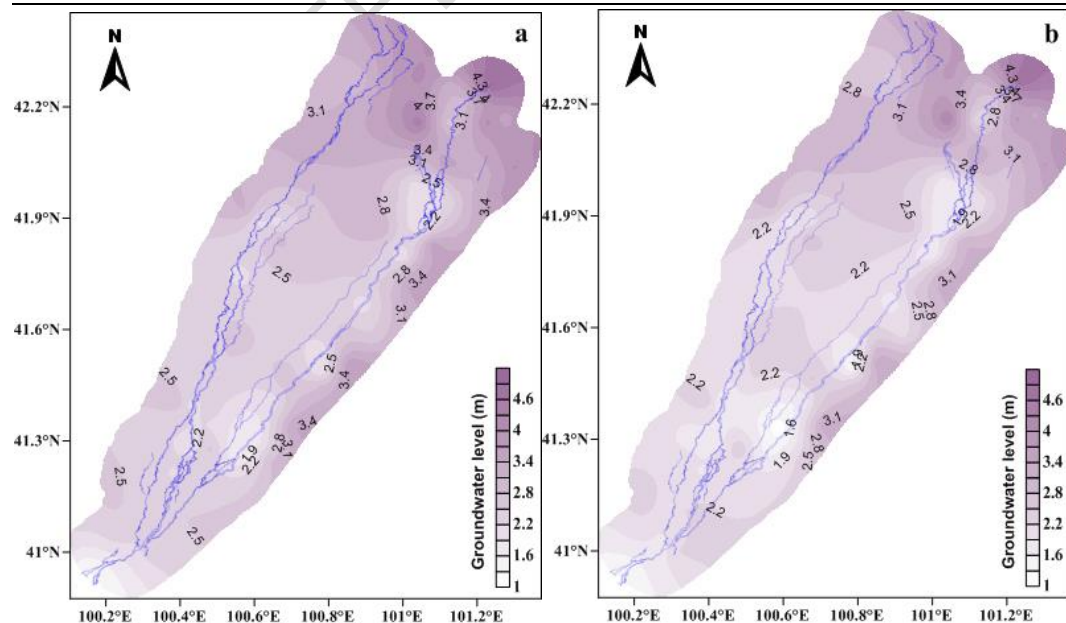
Fig. 5 The spatial change of groundwater level in study area (a- before eco-water diversion project; b- after eco-water diversion project)
