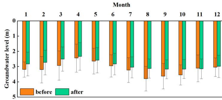
Fig. 6 The monthly variation of groundwater level in study area(before- before eco-water diversion project; after- after eco-water diversion project)
