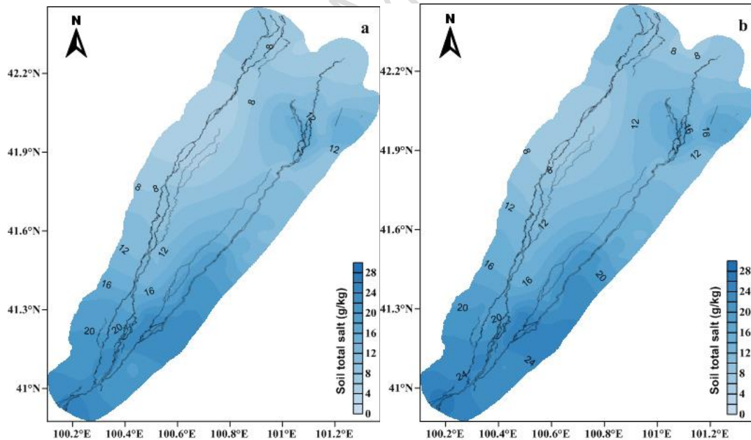
Fig. 7 The spatial change of soil salt content after eco-water diversion project in study area(a- before eco-water diversion project; b- after eco-water diversion project)
