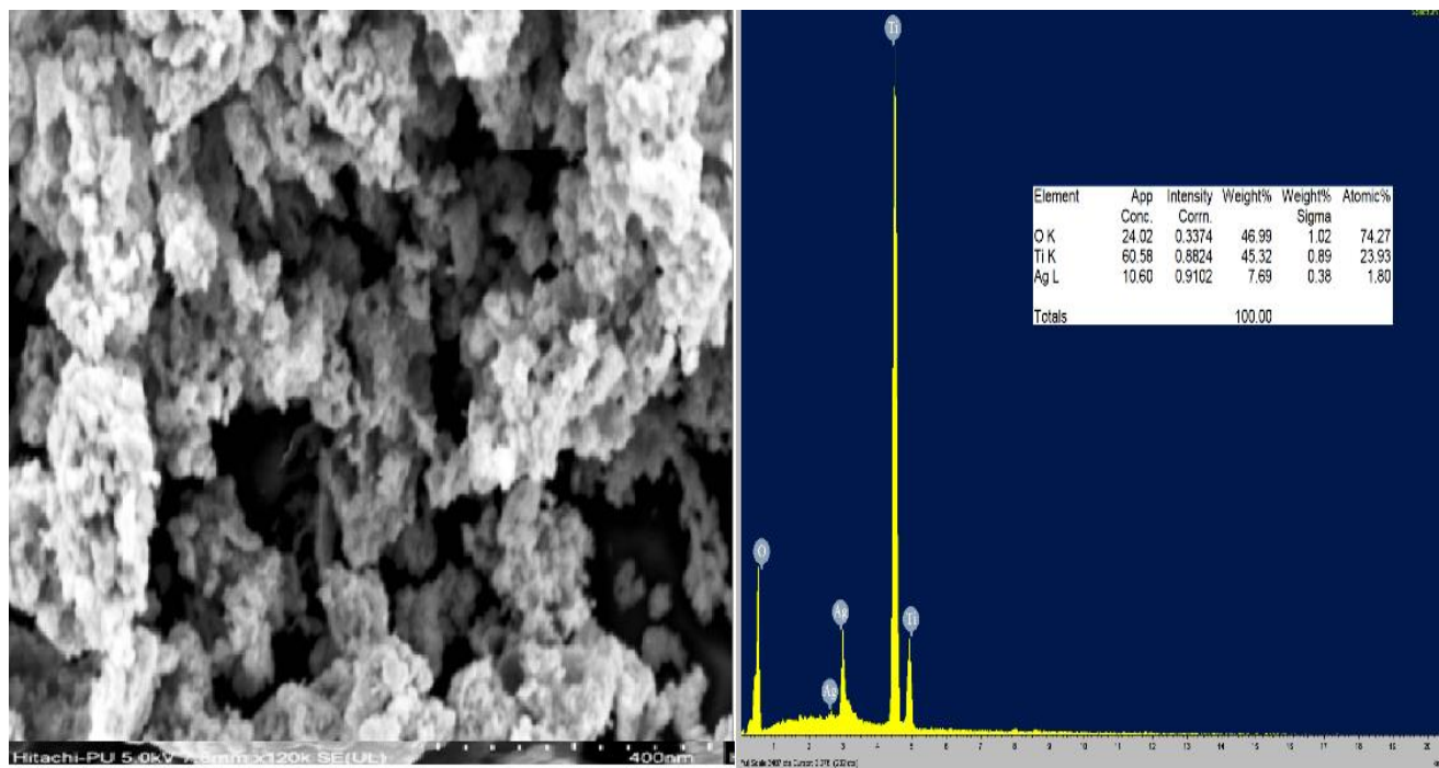
Figure 3a SEM and EDAX analysis of Ag/TiO 2
