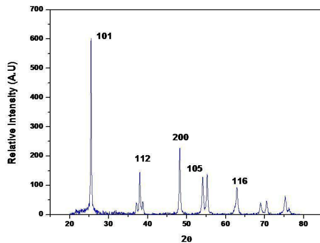
Figure 2 X-Ray Diffraction patterns of Ag/TiO 2 Nanocomposites
