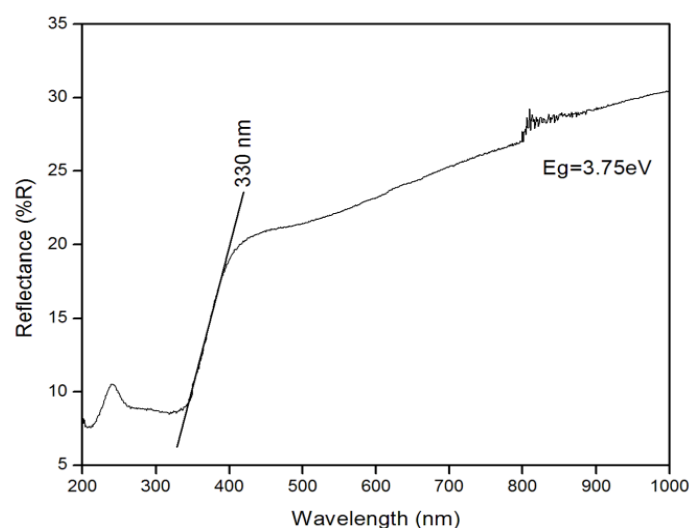
Figure 5 UV-DRS analysis of Ag/TiO 2
