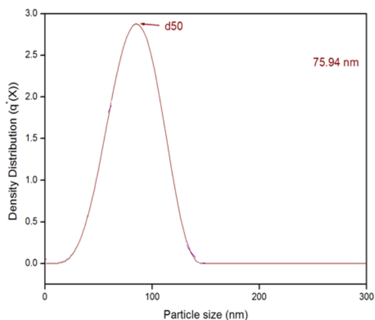
Figure 4 Particle size distribution of Ag/TiO 2
