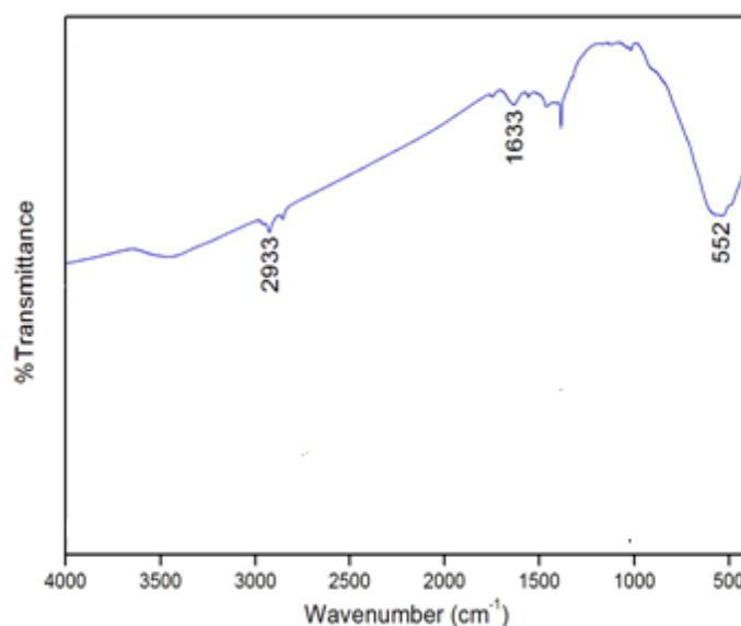
Figure 3 FTIR spectrum of Ag/TiO 2
