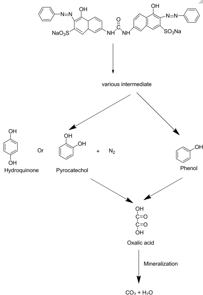
Figure 8. Degradation mechanism of direct orange 26 dye.
