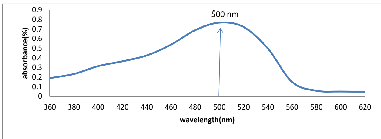
Figure 4. Determination of \lambda_{\max} for Direct Orange 26 dye.
