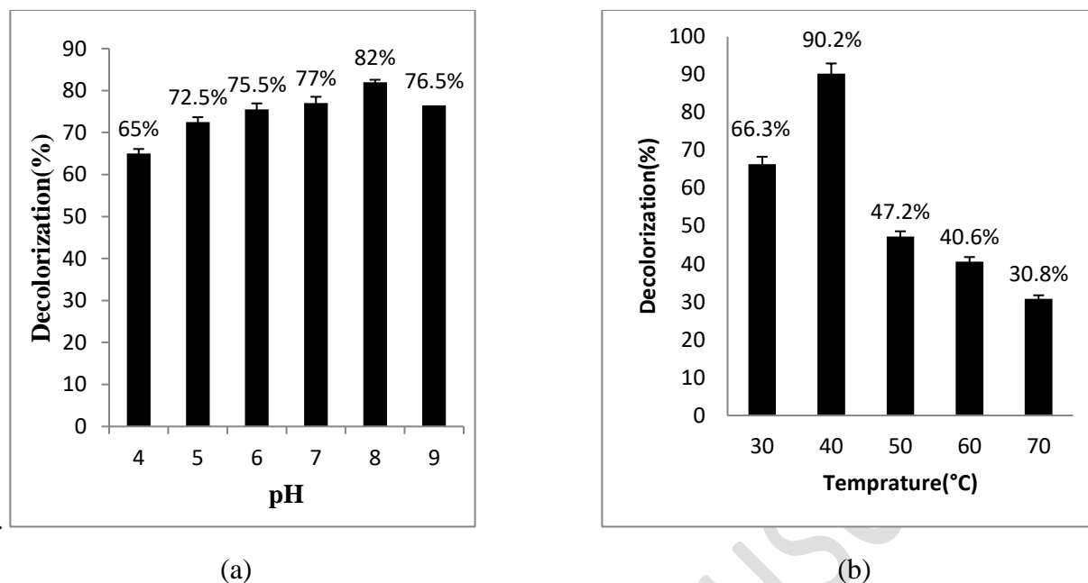
Figure 6. pH effect on direct orange 26 dye decolorization with Cu nanoparticles (a) Temperature effect on decolorization of direct orange 26 dye engaging Cu-NPs (b).
