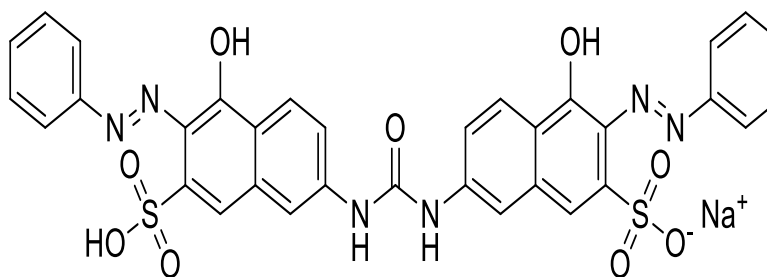
Figure 1. Structure of Direct Orange 26 dye
