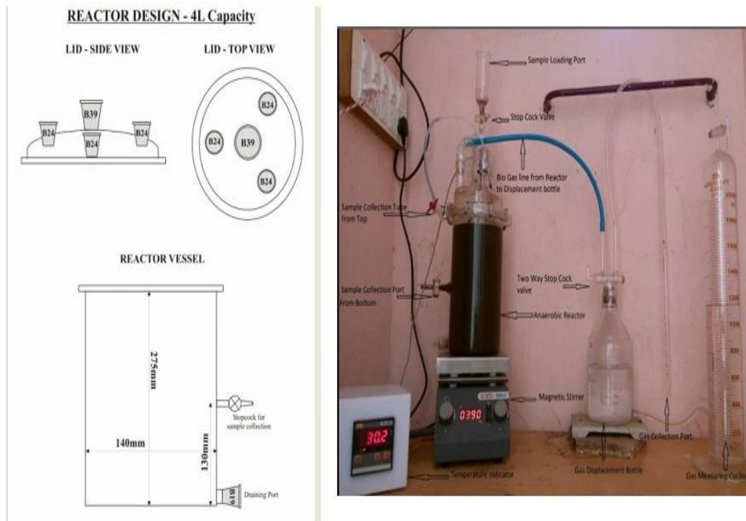
Fig 2: Experimental setup of biogas production
