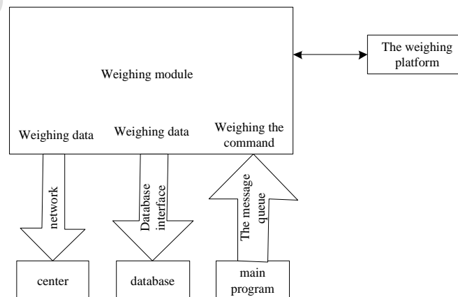
Figure 6. Block diagram of automatic weighing
