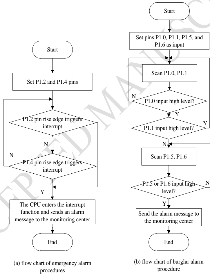
Figure 7. Flow chart of abnormal alarm program
