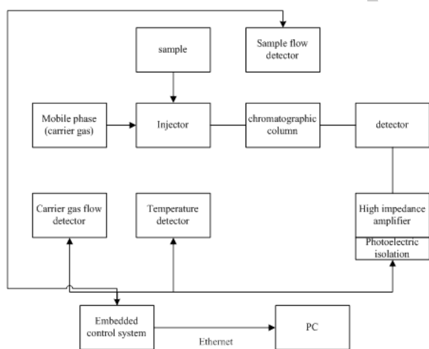
Figure 2. Basic principle block diagram of gas chromatograph technology
