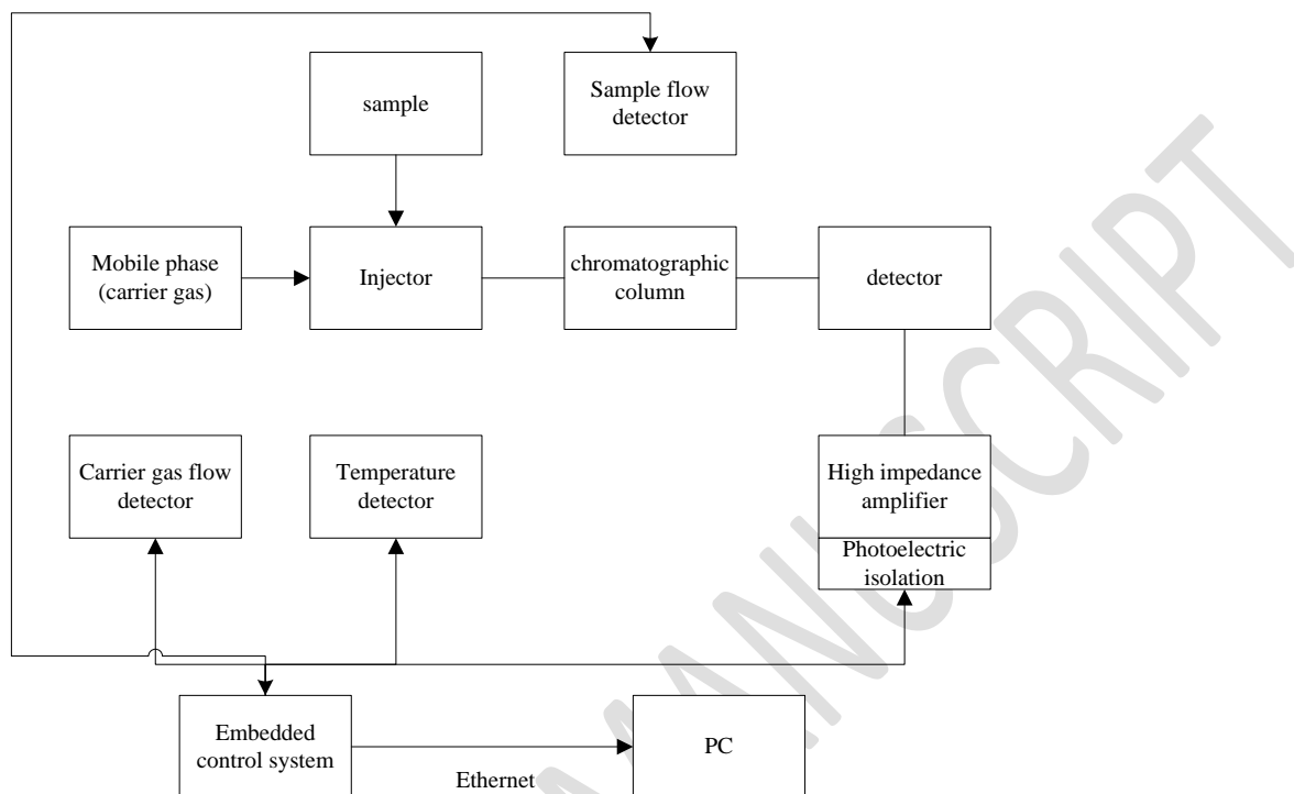
Figure 2. Basic principle block diagram of gas chromatograph technology
