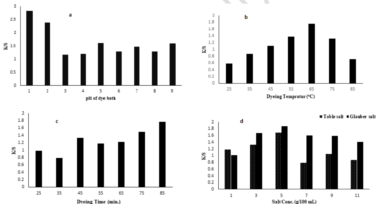
Figure 3. Effect of different dyeing parameters (a) pH of dye bath (b) Dyeing temperature (c) Dyeing time (d) Salt concentrations on the optimum wool, dyed fabric 1 min. irradiated wool and irradiated extract (RW/RE) under the microwave treatment
