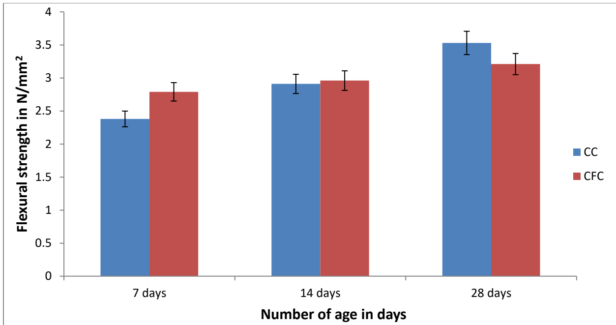
Figure 7. Flexural Strength relations between CC and CFC Samples
