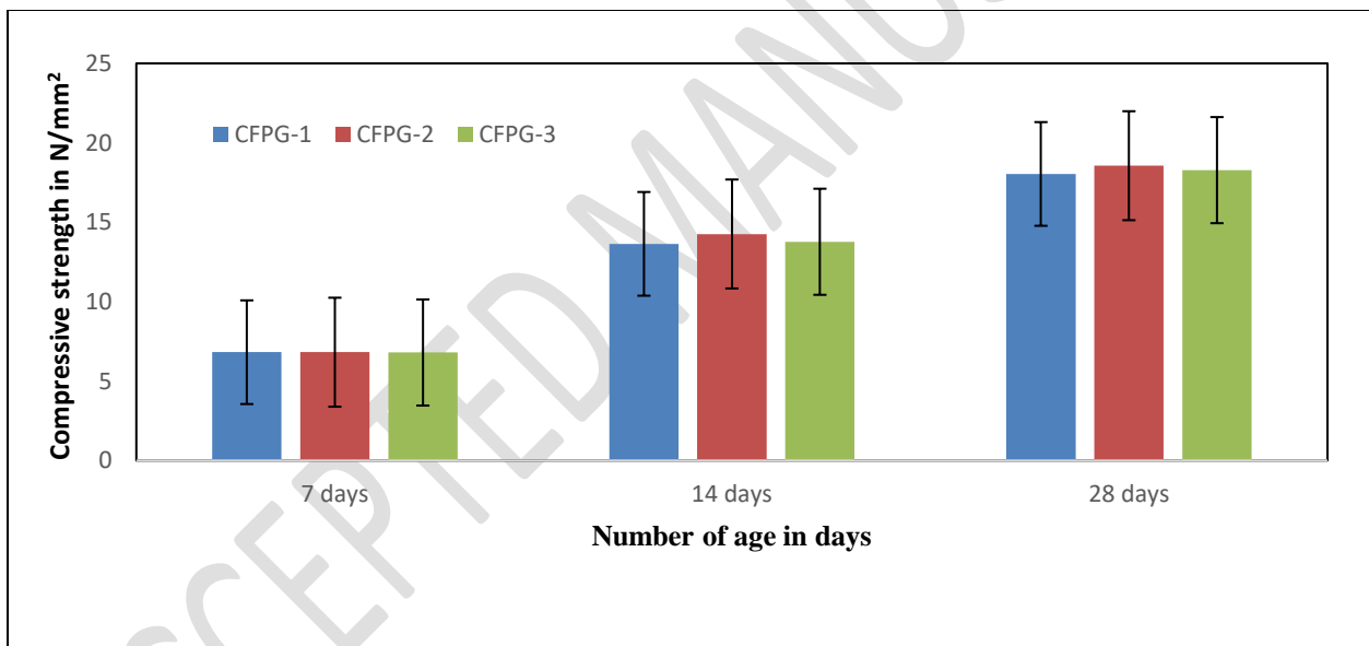
Figure 4. Compressive Strength relations between CFPG-1, CFPG-2 & CFPG-3 Samples with ages
