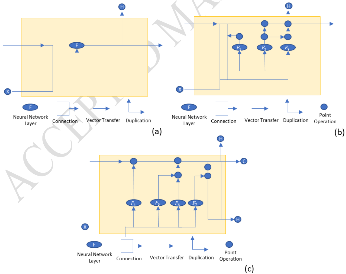
Figure 2. Block system of (a) RNN, (b) GRU and (c) LSTM models (Rathor, 2018)
