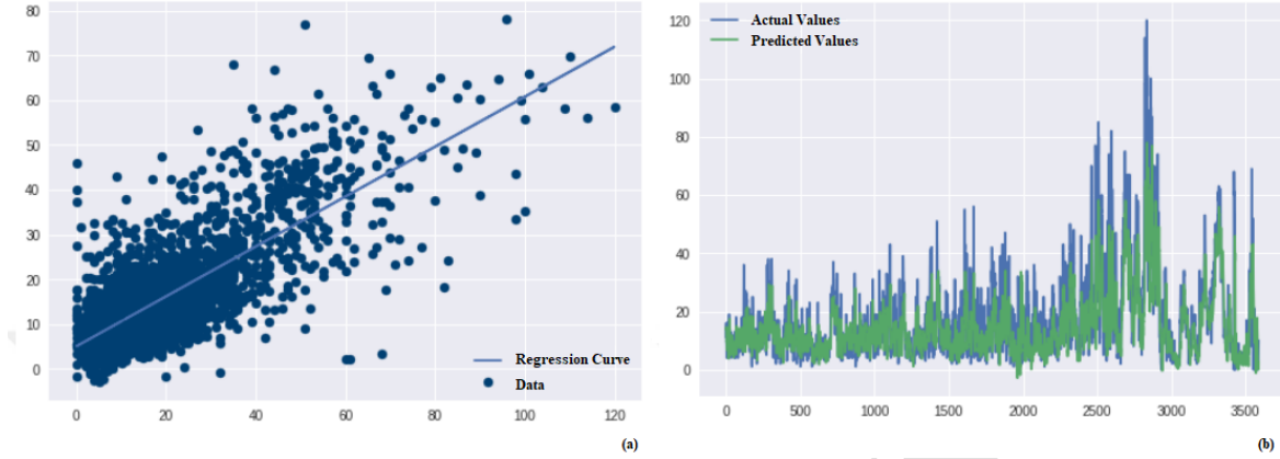
Figure 7. (a) Regression curve of actual (y-axis) and predicted (x-axis) values for three-hour prediction (b) Comparison of actual and predicted results (y-axis) with respect to time in seconds (x-axis) for three-hour prediction
