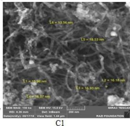
Figure.3. Field emission scanning electron microscopy (FE-SEM) image.(A1)MWCNT, (C1) Ni-Pt/ MWCNT That 5%W.Pt and 15%W.Ni , (B1) Ni-Pt/MWCNT That 3%W.Pt and 25%W.Ni.energy dispersive X-ray spectroscopy (EDS) spectra of catalyst(A2) MWCNT (C2)Ni-Pt/ MWCNT That 5% W.Pt and 15%.W.Ni , (B2) Ni-Pt/ MWCNT That 3%W.Pt and 25%.Ni.
