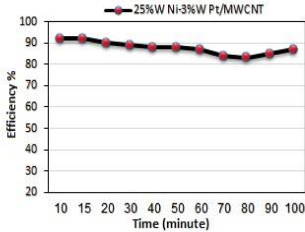
Figur.9. NO_2 removal efficiency profiles over prepared catalyst 25% W.Ni-3% W.Pt based on MWCNT. Concentration NO_2 3000 ppm and Space Velocity 25000/hr.
