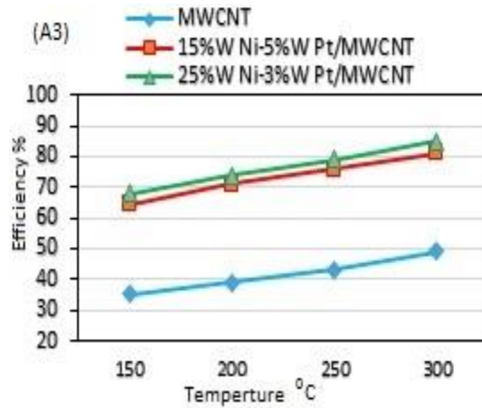
Figur.6. NO_2 removal efficiency profiles over prepared catalysts MWCNT, 15%W.Ni-5% W.Pt/MWCNT, 25% W.Ni-3% W.Pt/MWCNT at a space velocity of 25000/hr and temperature 150, 200, 250, 300 °C and (A1) concentration of 3000ppm (A2) concentration of 4000 ppm (A3)concentration of 5000 ppm.
