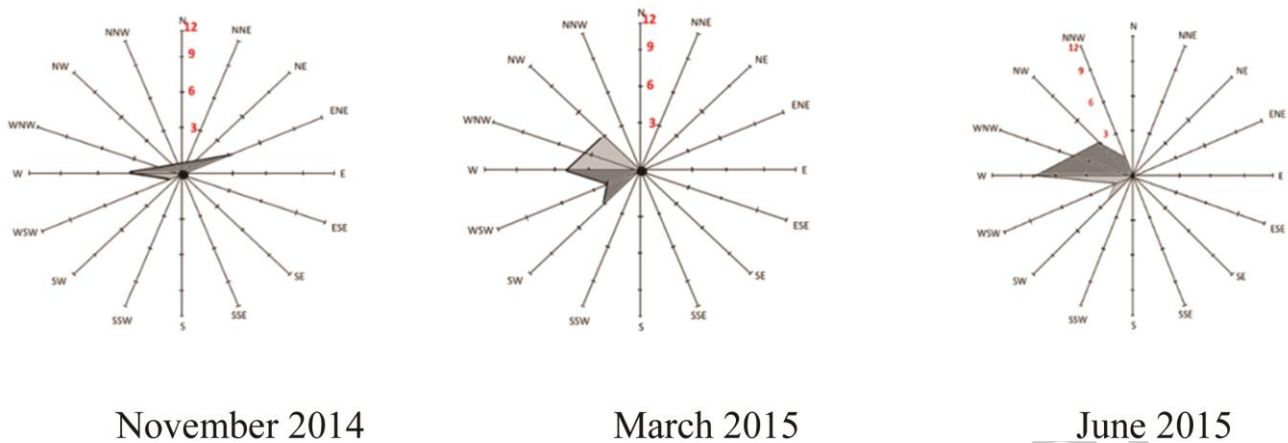
Figure 4. Prevailing wind direction in different season
