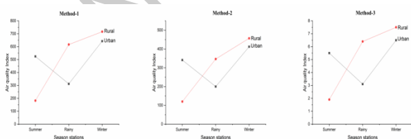
Figure 9. AQI comparison
