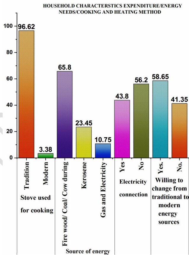
Figure 7. Energy usage pattern in rural houses
