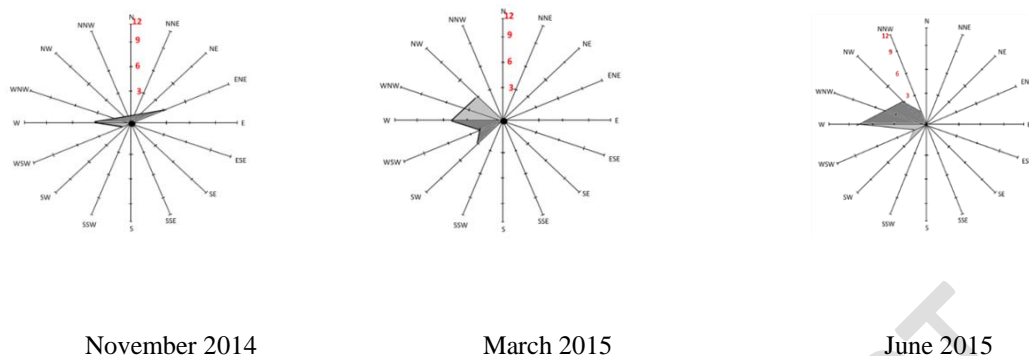
Figure 4. Prevailing wind direction in different season
