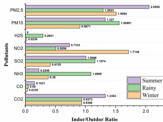
Figure 5. Indoor/Outdoor ratio for various pollutants in urban environment
