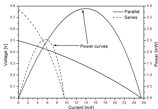
Figure 4. Power and polarization curves for the stack under series connection and parallel connection
