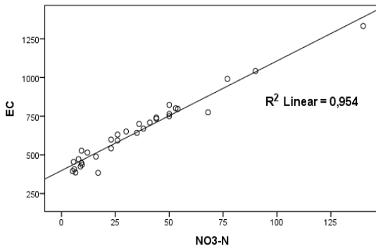
Figure 2. Relationship of soil electrical conductivity and soil \text{NO}_3\text{-N}
