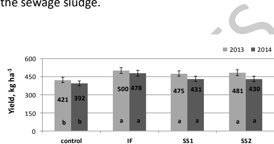
Figure 1. Influence of MSS application on cotton yield (for each year, different letters indicate statistically significant difference at probability level p < 0.05 according to the LSD test)
