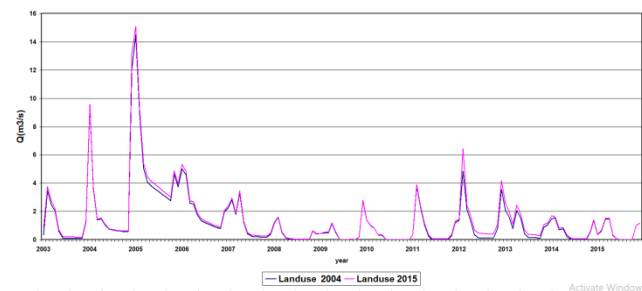
Figure 6. Monthly discharge Hydrograph from 2003 to 2015 in the Chenar Rahdar watershed
