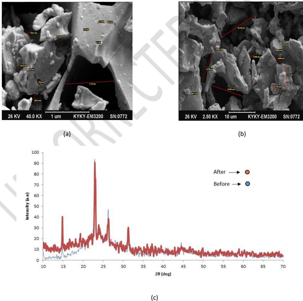
Figure 2. SEM micrographs AC, a) unmodified, b) modified and c) XRD spectrum AC for before and after modified by ZnO
