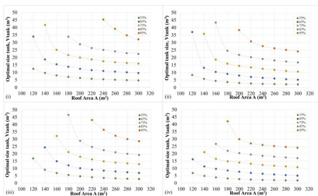
Figure 6. Optimal rainwater tank size for certain reliabilities to meet the percentage of p = 35\% of total daily demand for number of capita N_{\text{cap}} = 4 and 120 L/capita/day daily water use by using: (i) historical timeseries; (ii) 'a'; (iii) 'b'; and (iv) 'c' synthetic timeseries
