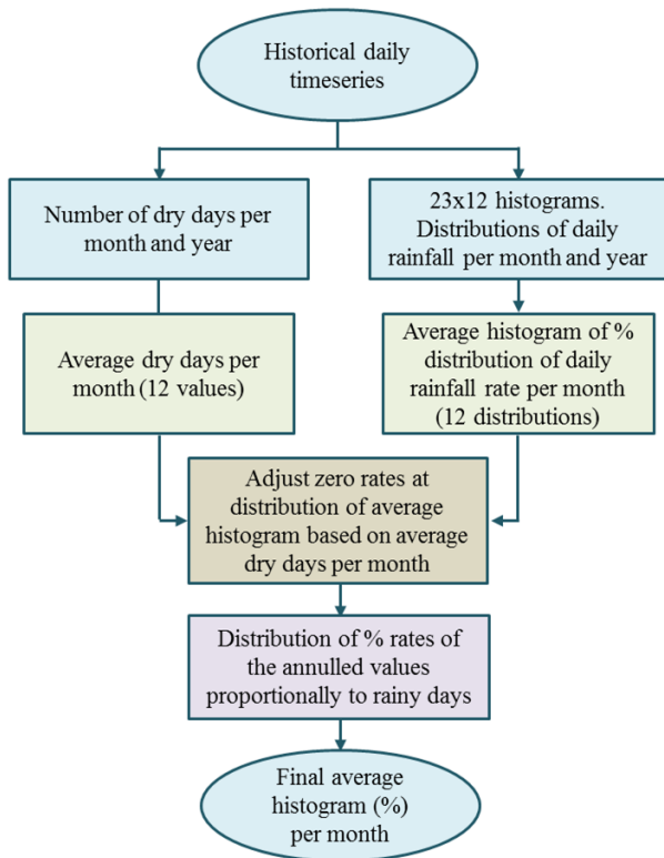
Figure 3. Disaggregation procedures for the generation of daily timeseries
