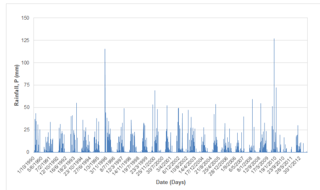
Figure 2. Historical daily rainfall data series from the nearest meteorological station (period: 1990-2012)
