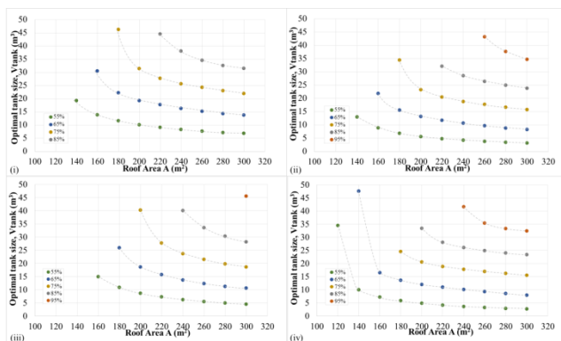
Figure 5. Optimal rainwater tank size for certain reliabilities to meet the percentage of p = 35\% of total daily demand for number of capita N_{\text{cap}} = 4 and 150 \text{ L/capita/day} daily water use by using: (i) historical timeseries; (ii) 'a'; (iii) 'b'; and (iv) 'c' synthetic timeseries
