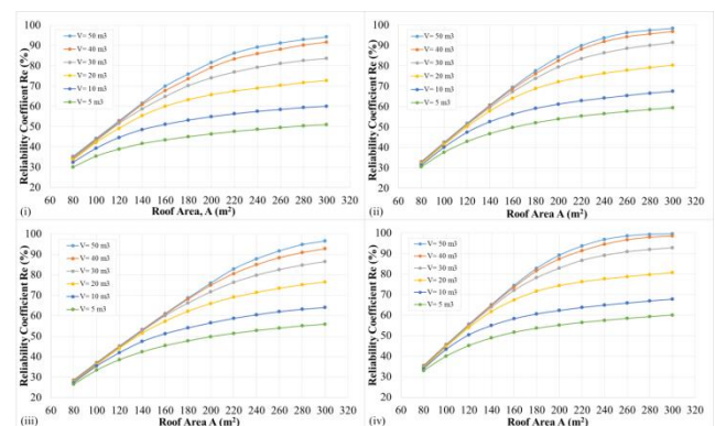
Figure 4. Reliability coefficient for different ranges of roof area and rainwater tank volumes for: (i) the historical record; (ii) the synthetic timeseries ‘a’; (iii) the synthetic timeseries ‘b’; and (iv) the synthetic timeseries ‘c’
