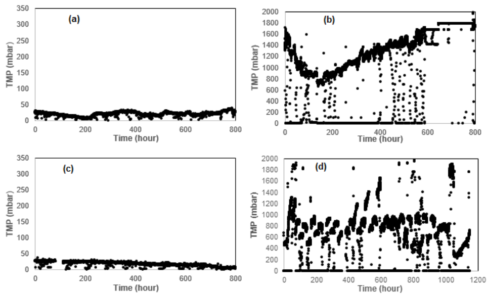
Figure 6. TMP of (a) V-PSUF and (b) P-PSUF combination with sedimentation, and (c) V-PSUF and (d) P-PSUF combination with filtration of Emirli treatment plant
