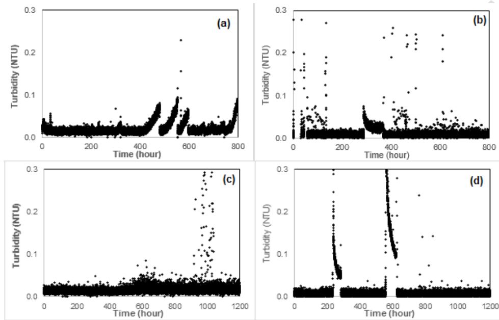
Figure 2. Effluent turbidity values of (a) V-PSUF and (b) P-PSUF combination with sedimentation and (c) V-PSUF, (d) P-PSUF combination with filtration in Büyükkçekmece treatment plant
