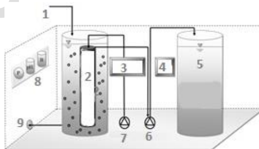
Figure 1. Schematic diagram of membrane systems: 1) Raw water, 2) Membrane module, 3) Data logger, 4) PLC, 5) Clean water tank, 6) Vacuum and recycling pump, 7) Air pump, 8) Pressure, pH and turbidity meters, 9) Discharge
