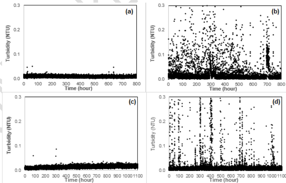
Figure 3. Effluent turbidity values of (a) V-PSUF and (b) P-PSUF combination with sedimentation and (c) V-PSUF, (d) P-PSUF combination with filtration in Emirli treatment plant
