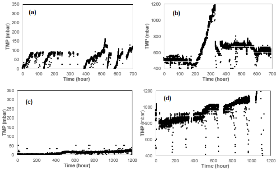
Figure 5. TMP of (a) V-PSUF and (b) P-PSUF combination with sedimentation, and (c) V-PSUF and (d) P-PSUF combination with filtration in Büyükçekmece treatment plant
