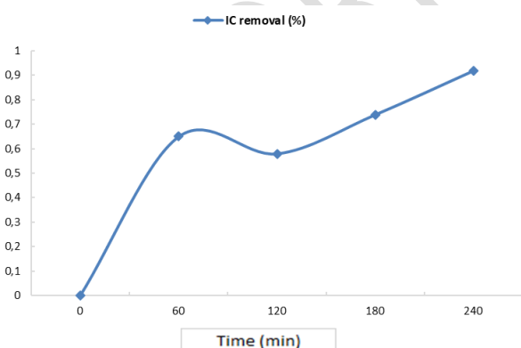
Figure 3. Variation in degradation rate of inorganics carbon (IC) during the solar photo-catalyst of \text{TiO}_2/\text{ZnO}/\text{Fenton} process at pH 7
