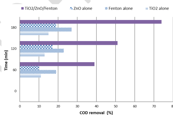
Figure 4. Comparing treatment time of the solar photocatalyst \text{TiO}_2/\text{ZnO}/\text{Fenton} process with different processes under pH 7.
