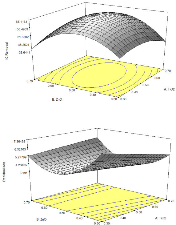
Figure 2. Response surface models for IC removal efficiencies and residual iron (RI) by the solar photocatalyst of \text{TiO}_2/\text{ZnO}/\text{Fenton} process
