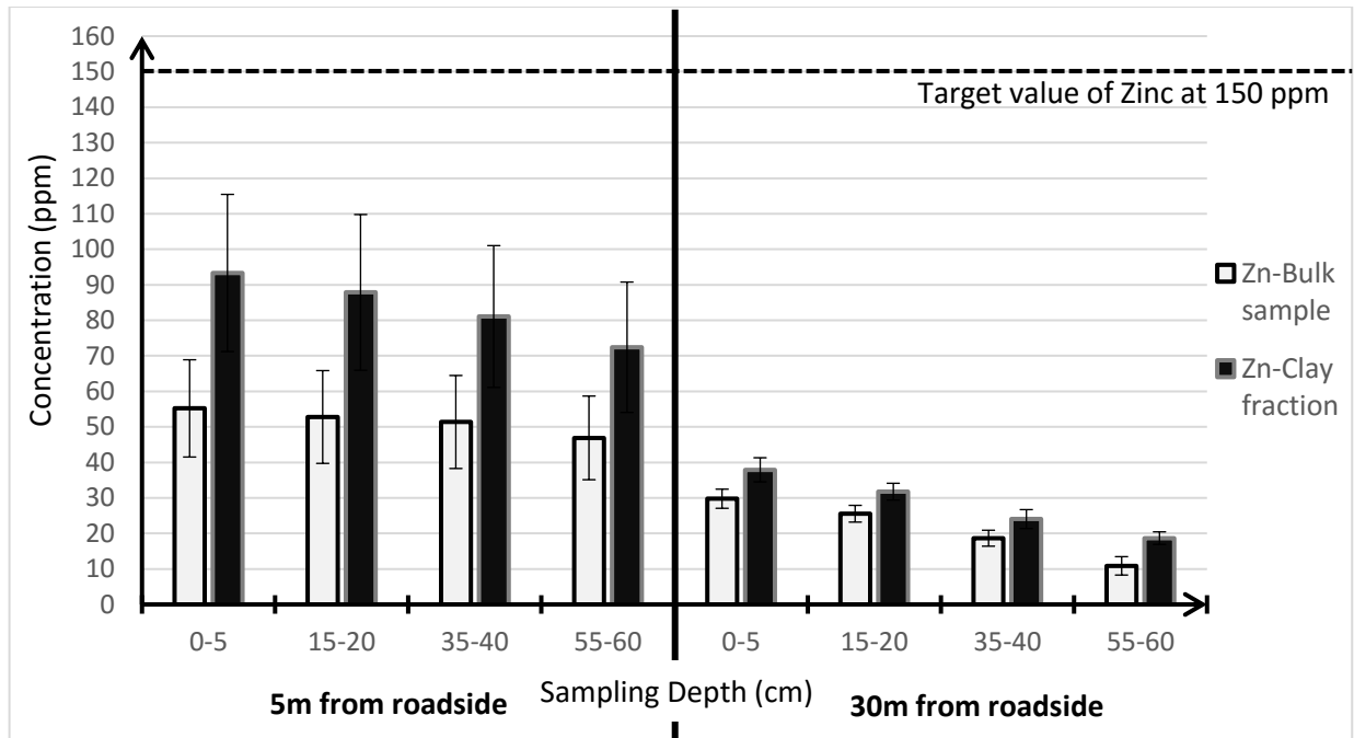
Figure 7a. Mean concentration of zinc with standard deviation error bars for bulk sample and clay fraction in roadside soil along Ilesa-Akure road with respect to depth and distance.
