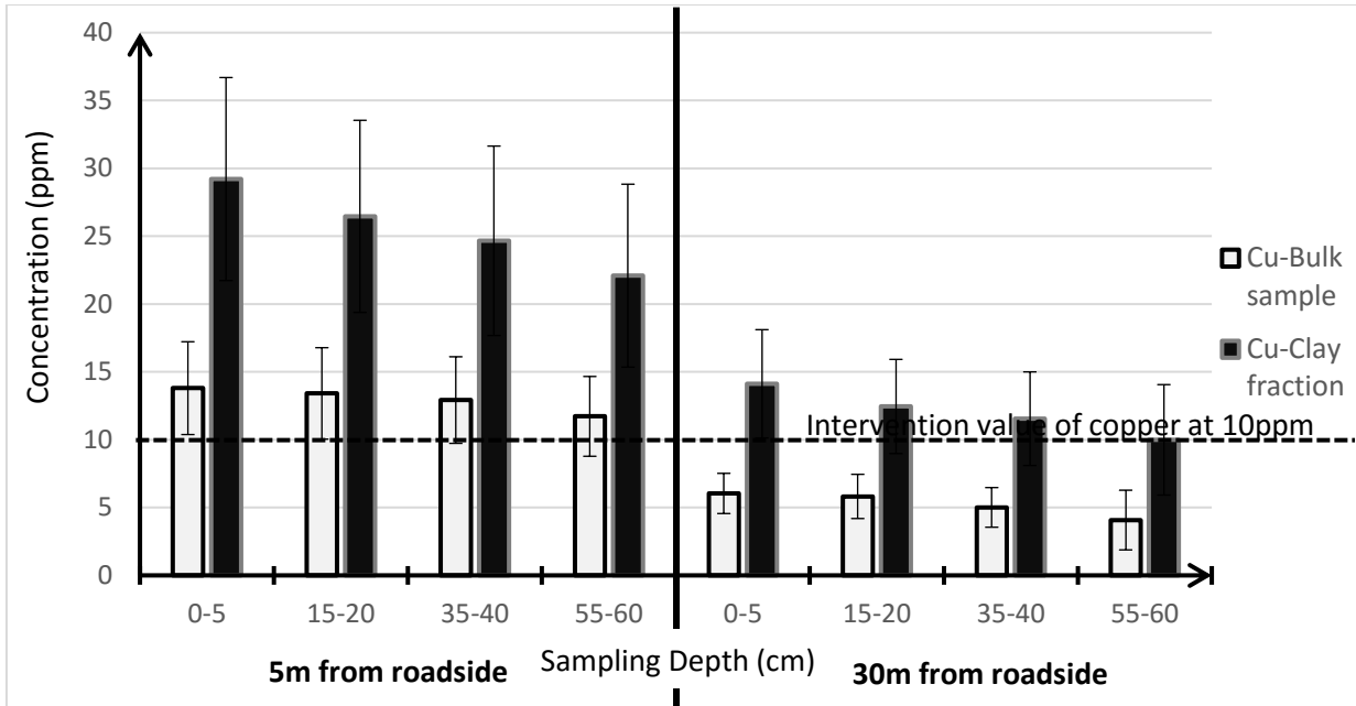
Figure 9a. Mean concentration of copper with standard deviation error bars for bulk sample and clay fraction in roadside soil along Ilesa-Akure road with respect to depth and distance
