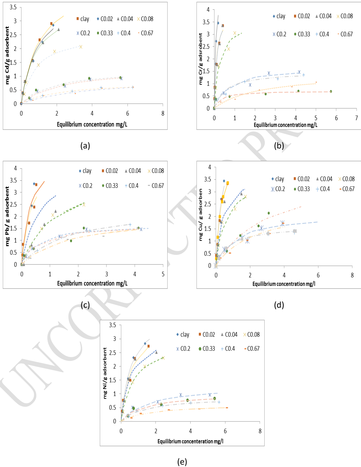
Figure 1. Adsorption isotherm of the prepared modified bentonite for different metals (a) cadmium, (b) Chromium, (c) Lead, (d) copper and (e) Nickel.
