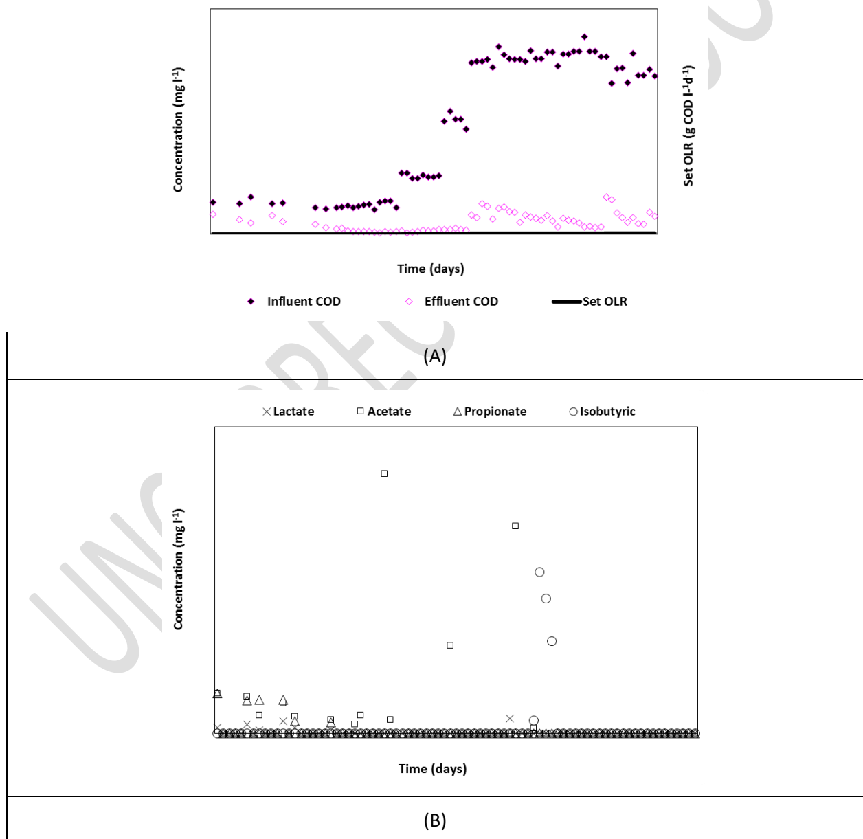
Figure 1. Time courses in (A) COD removal and (B) effluent VFA of the UASB reactor symbol: set OLR-set organic loading rate
