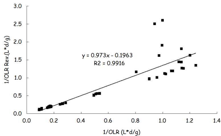
Figure 4. Stover-Kincannon model for COD removal in the UASB reactor
