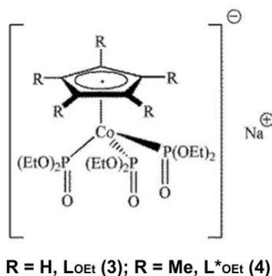
Figure 1. The molecular structure of NaLOEt (3) and NaL^*OEt (4).
