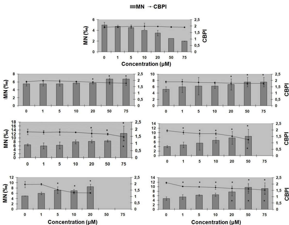
Figure 2. Induction of MN and CBPI values in human lymphocytes treated with a \text{SnCl}_2 \cdot 2\text{H}_2\text{O} (1), b \text{NaLOEt} (3), c \text{NaL}^*\text{OEt} (4), d \text{LOEtSnCl} (5), e \text{L}^*\text{OEtSnCl} (6), f \text{LOEtSnPh}_3 (7) and g \text{L}^*\text{OEtSnPh}_3 (8). 4000 binucleated cells scored per experimental point, * p < 0.05 [G-test for MN]; * p < 0.001 [ \chi^2 for CBPI]
