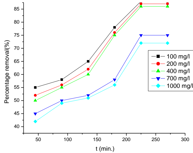
Figure 4. Effect of contact time on removal of 2,4-DCP onto MSAC (Adsorption study) (At adsorbent dose 10 g l -1 and pH 7)
