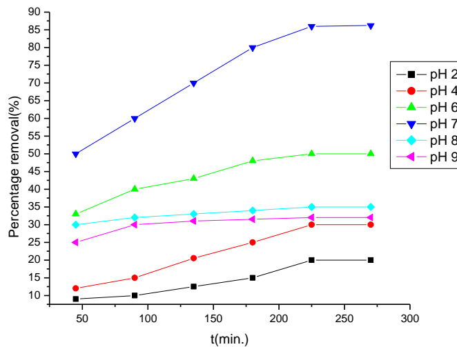
Figure 2. Effect of pH on removal of 2,4-DCP onto MSAC (Adsorption study) (At initial conc. 400 \text{ mg l}^{-1} and adsorbent dose 10 \text{ g l}^{-1} )
