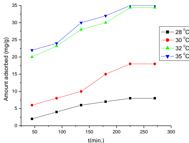
Figure 9. Effect of temperature on removal of 2,4-DCP onto MSAC (Adsorption study)(At pH 7, adsorbent dose 10 g l -1 , initial conc. 400 mg l -1 )
