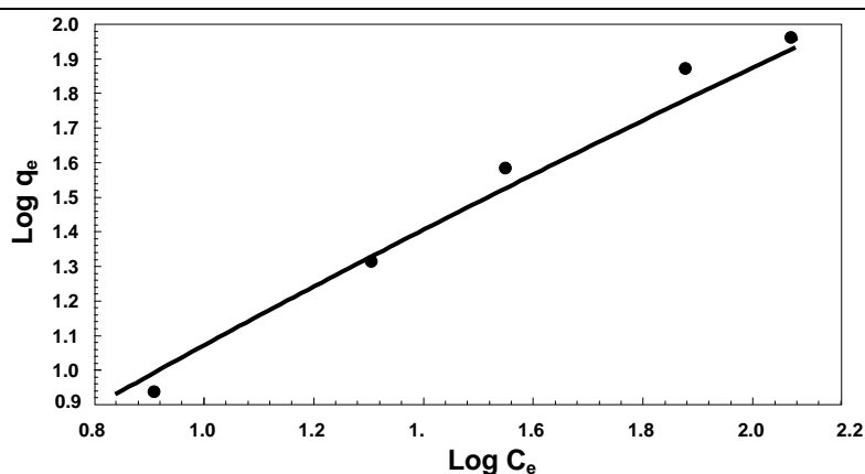
Figure 11. Freundlich isotherm for removal of 2,4-DCP onto MSAC (SAB study) (At pH 7 and adsorbent dose 10 \text{ g l}^{-1} )
