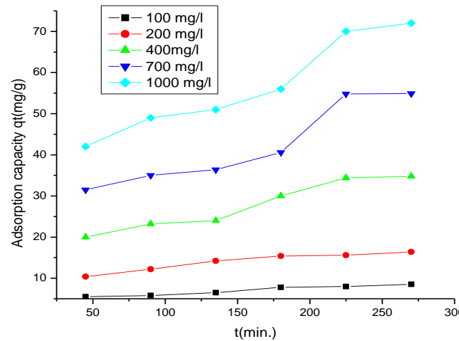
Figure 5. Effect of contact time on removal of 2,4-DCP onto MSAC (SAB study) (At adsorbent dose 10 g l -1 and pH 7)
