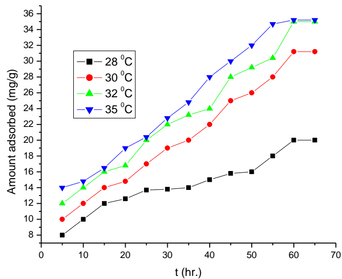
Figure 8. Effect of temperature on removal of 2,4-DCP onto MSAC (SAB study) (At pH 7, adsorbent dose 10 g l -1 , initial conc. 400 mg l -1 )
