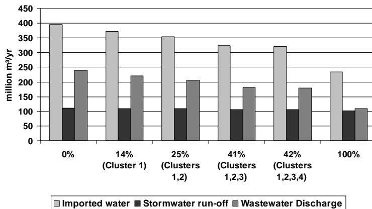
Figure 6. Performance of the on-site wastewater treatment option
