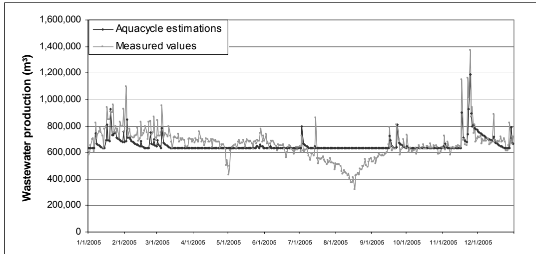
Figure 4. Measured and estimated wastewater production
