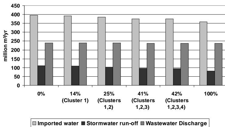
Figure 5. Performance of the rainwater use option
