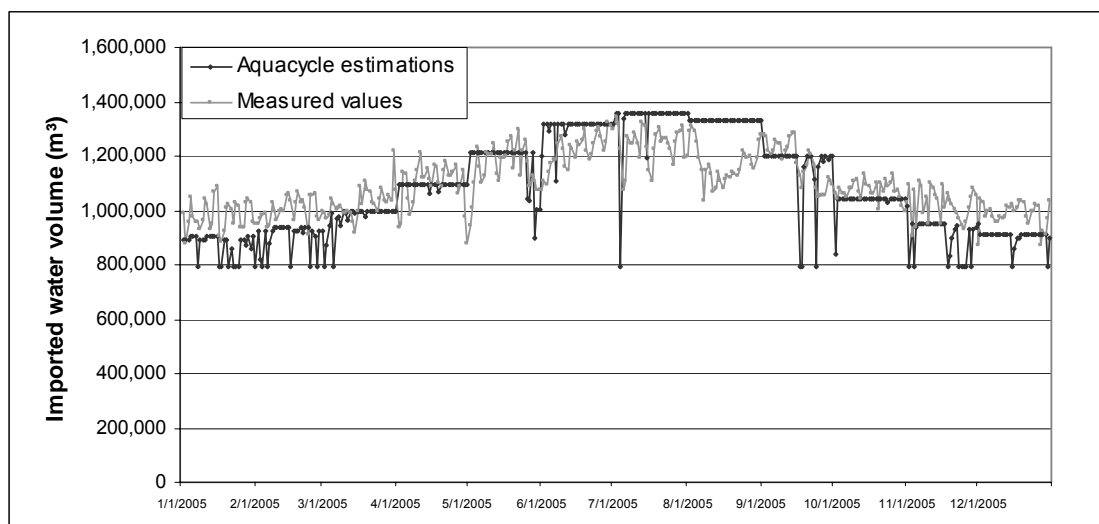
Figure 3. Measured and estimated imported water volumes
